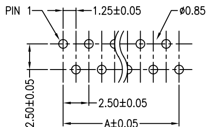
SPECIAL PCB LAYOUT
